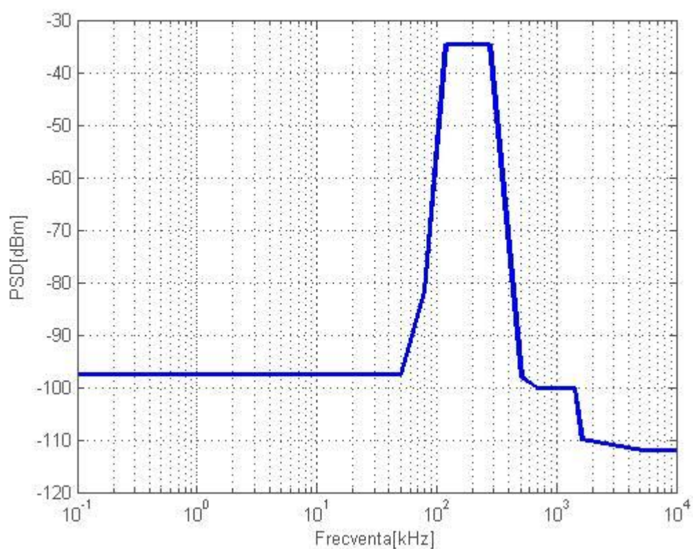
Exhibit 13 – PSD mask
